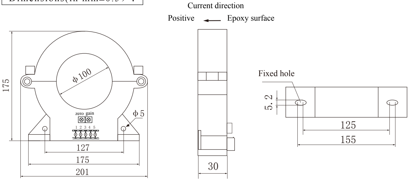
Connector Illustration:
