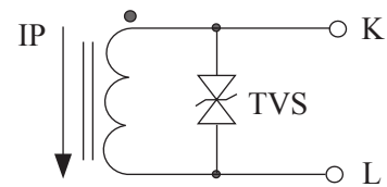
Built-in two-way protection diode Current output type
