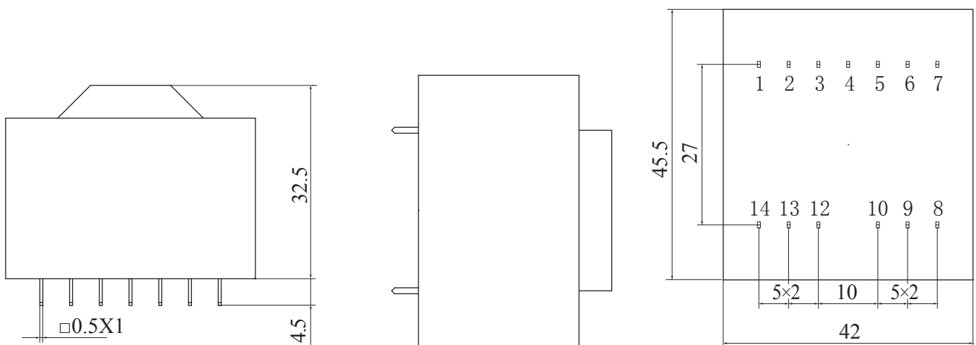
Front View
