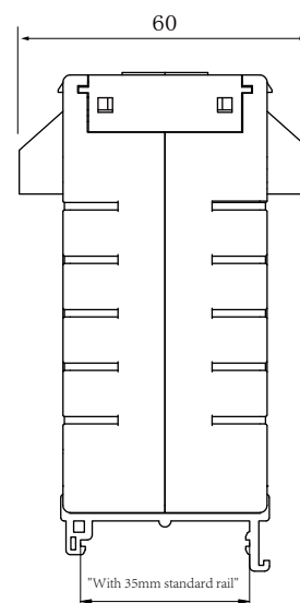
Installation diagram of clamp rail
