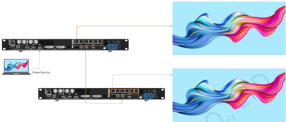
Figure 5-39 Copy
