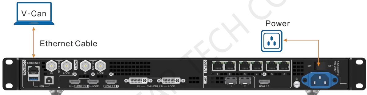
Figure 6-1 Hardware connection
