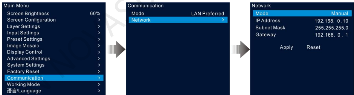
Figure 5-45 Network settings
