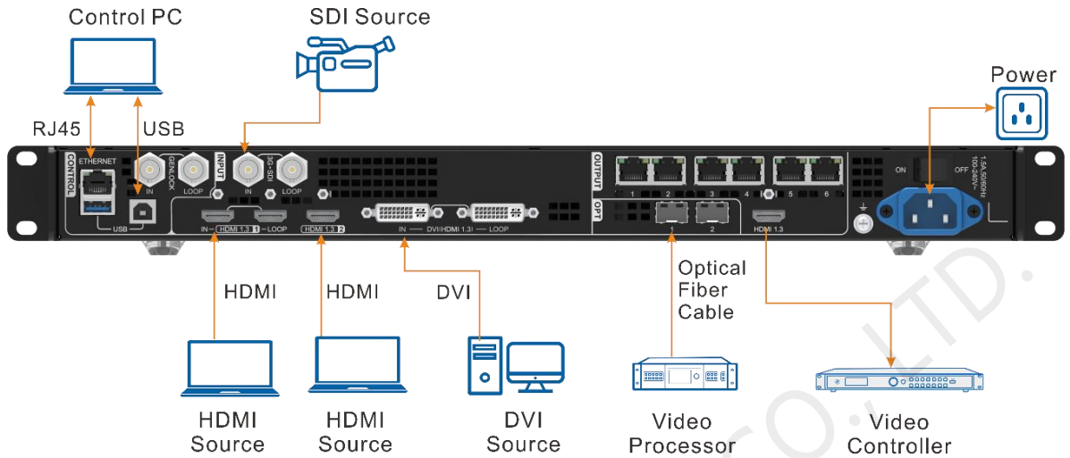
Figure 5-33 HDMI output
