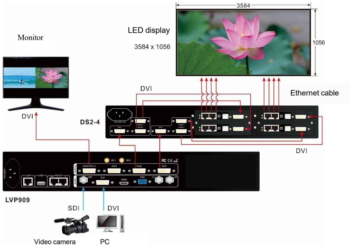
Diagram 4-2 Typical Application Connection Diagram
