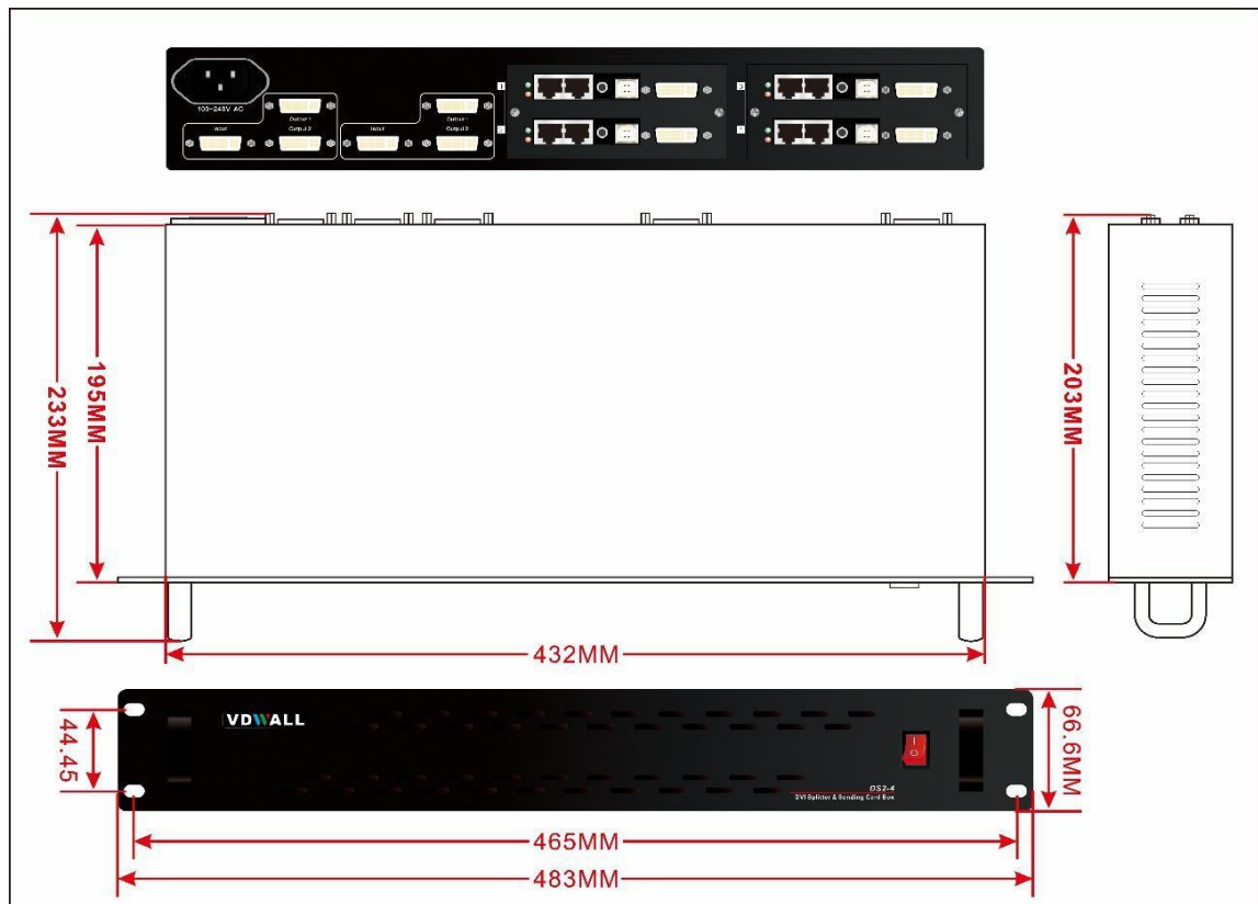
Diagram 4-4 Installation Dimension Diagram
