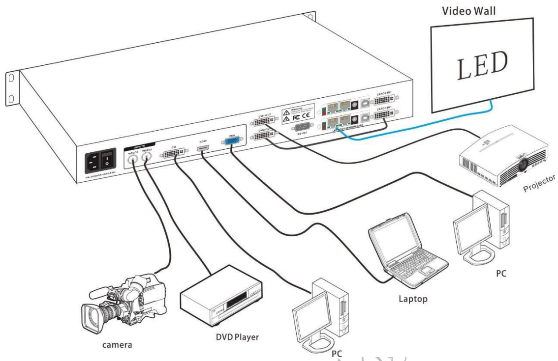
Connection diagram
