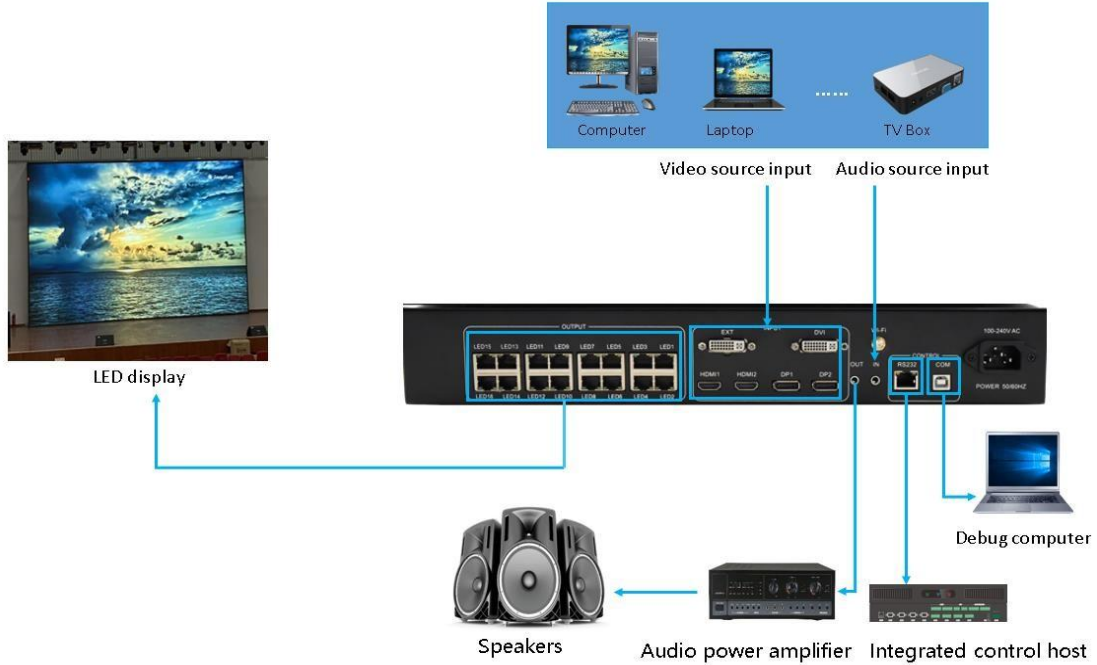
Connection diagram
