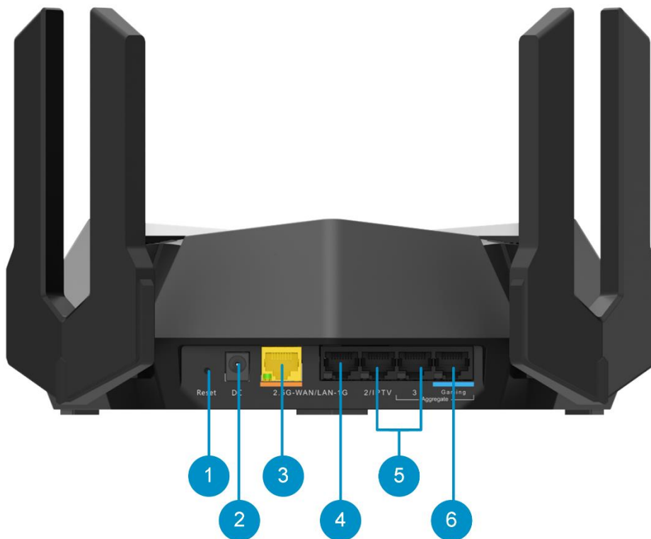
Figure 1-4 Back View
