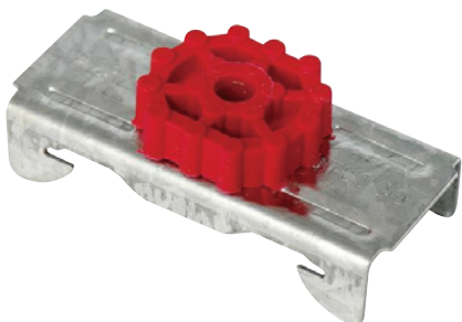
RESILIENT MOUNT CLIP CONCRETE RESILIENT MOUNT RED-ACOUSTIC ISO DFC TO SUIT FC
