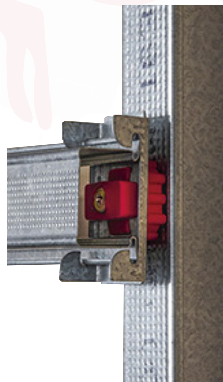
DIRECT FIX CLIP CEILING ADJUSTABLE
