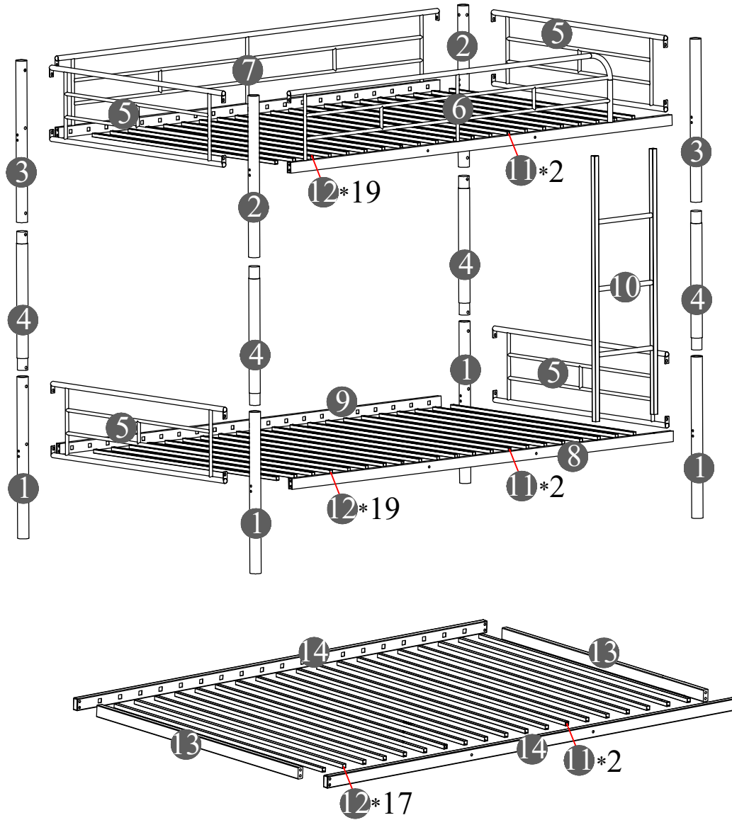
DETAIL VIEW
