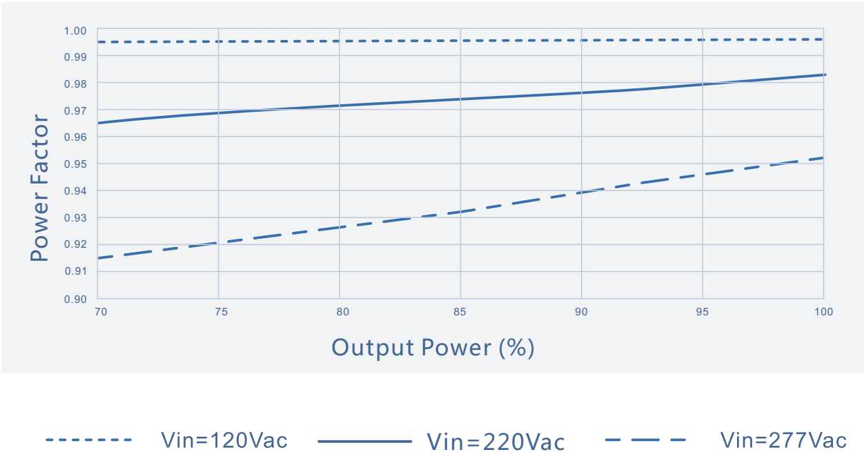
Power Factor Vs. Output Power
