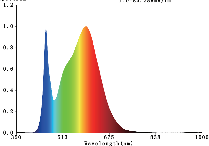
Spectrum
