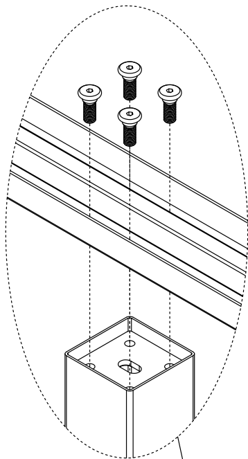
A. 3/4" Medium Machine Screw - 8
