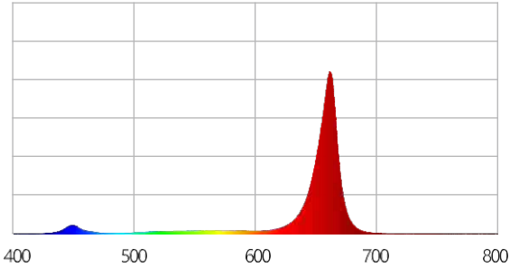
Full Spectrum GRAPH
