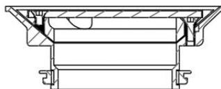
Cross Section
