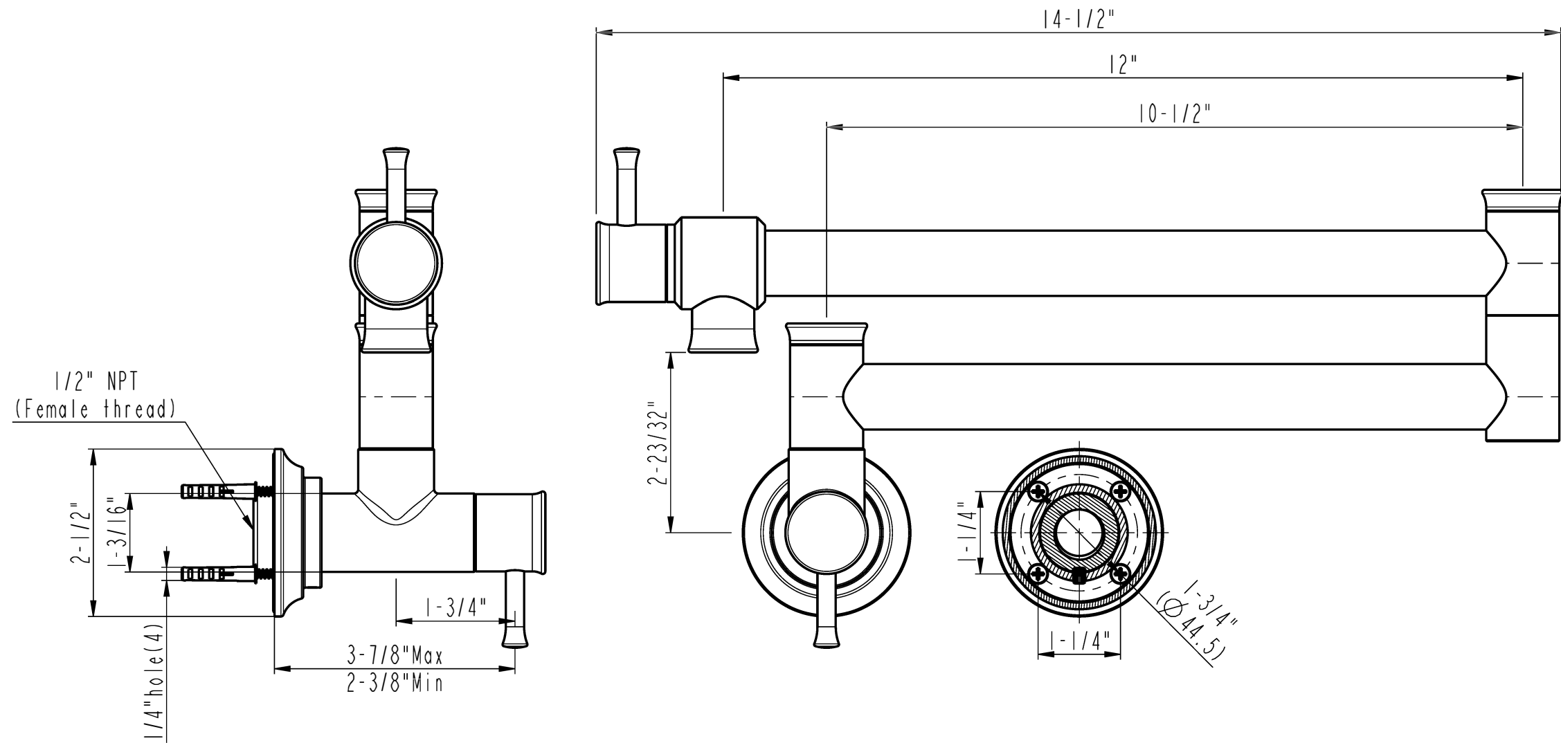
98266 Specifications
