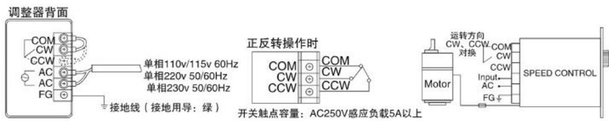
控制器接线图 Connection diagrams of the controller
