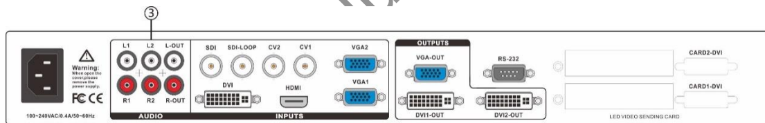
Figure 2—Audio Interface
