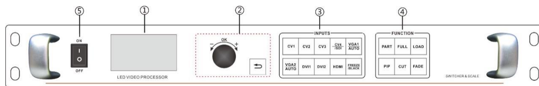
Figure 4-Front Panel
