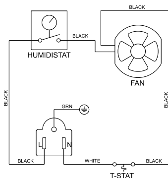
WIRING DIAGRAM
