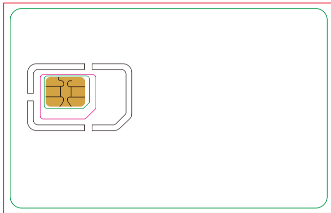
2FF/3FF front side with 8PIN Chip
