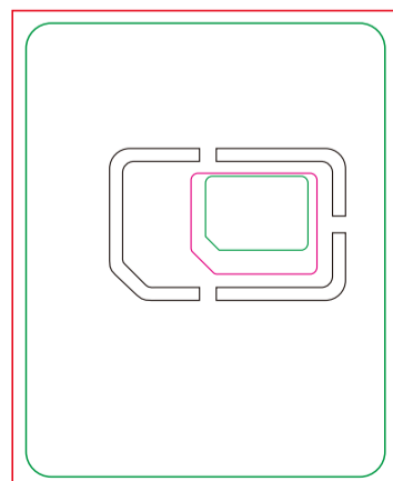
2FF/3FF/4FF back side
