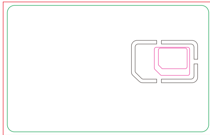
2FF/3FF/4FF back side
