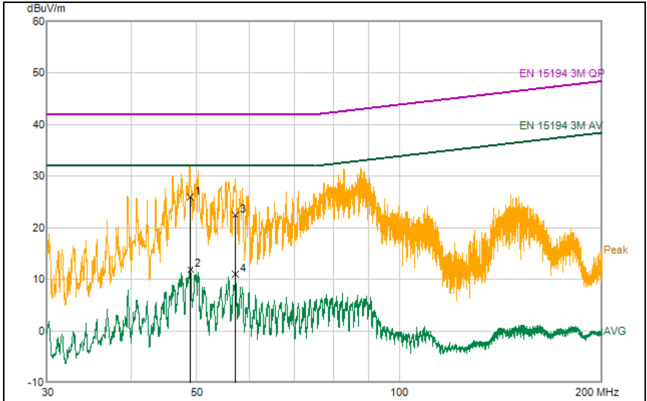
Figure 1: Spectral diagram and measurement results of broad-band radiated disturbance and narrow-band radiated disturbance, Vertical, 30MHz-200MHz
