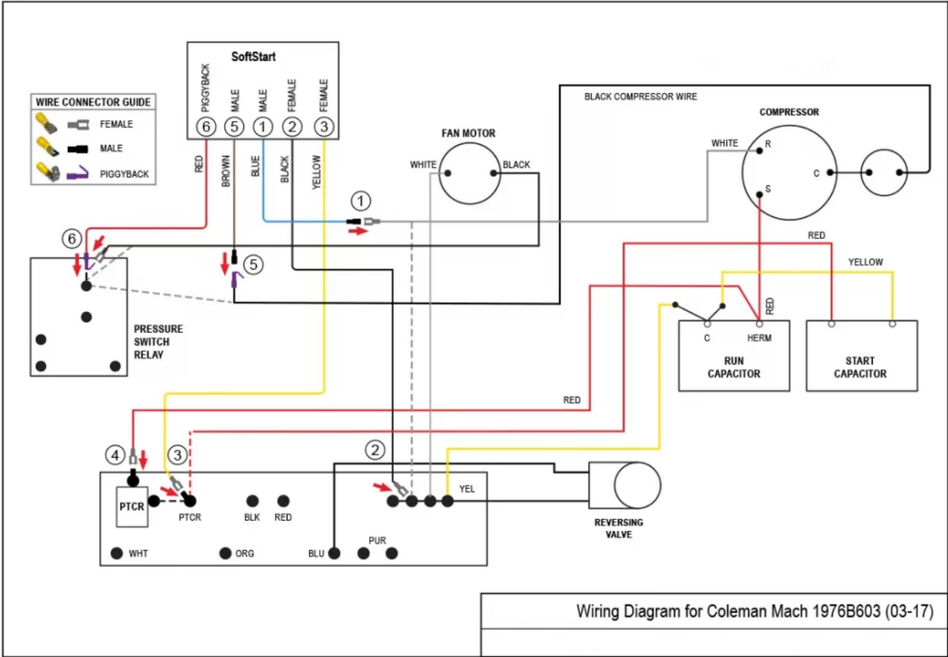
Wiring Diagram for Coleman Mach 1976B603
