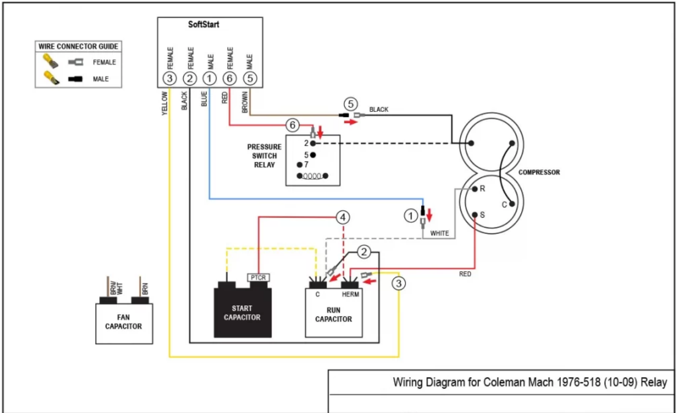
Wiring Diagram for Coleman Mach 1976-518
