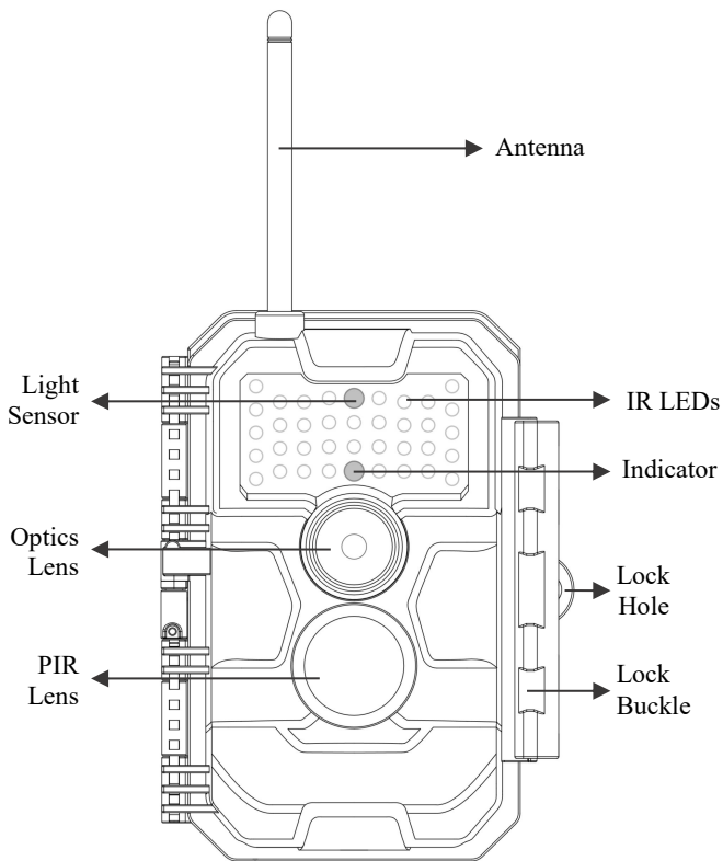
Figure 1: Front View
