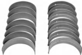
Conrod Bearing 460 030 0760
