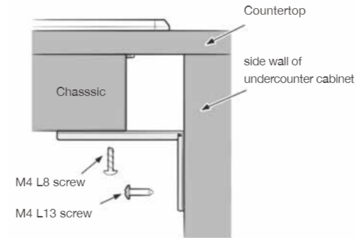
Installation Method 1
