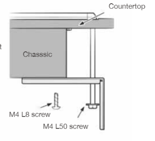
Installation Method 2
