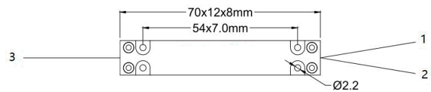
Slow axis working, Fast axis blocked Routing path is 3 to 1, 2(tap)
