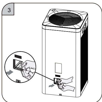
③ Pull out the sensor module by pulling the hardware.
