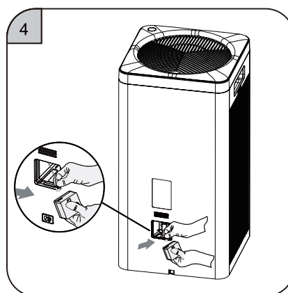
④ Pull out the terminal block from the old sensor module and replace it with a new sensor module.
