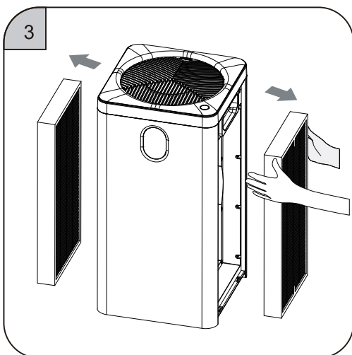
③ Take out the new filter screen with plastic film in the machine.
