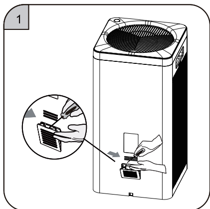
① Pry the sensor cover with a "—" shaped screwdriver.
