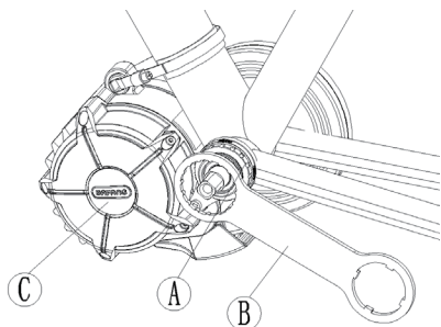
A Locking ring M33-PH1(B) B Special tool
