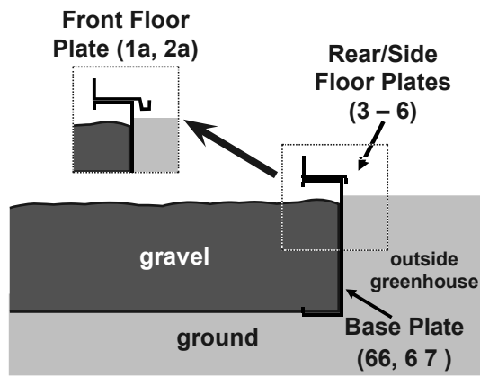
Cross Section
