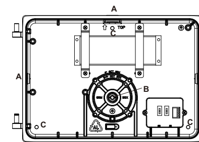
A - 1/2" NPS tapped holes ( surface conduit or photocell ) B - 1/2"NPS tapped holes C - 5/16" dia. screw hole
