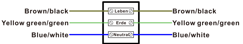
Bild. 3 Wiring diagram for input terminal
