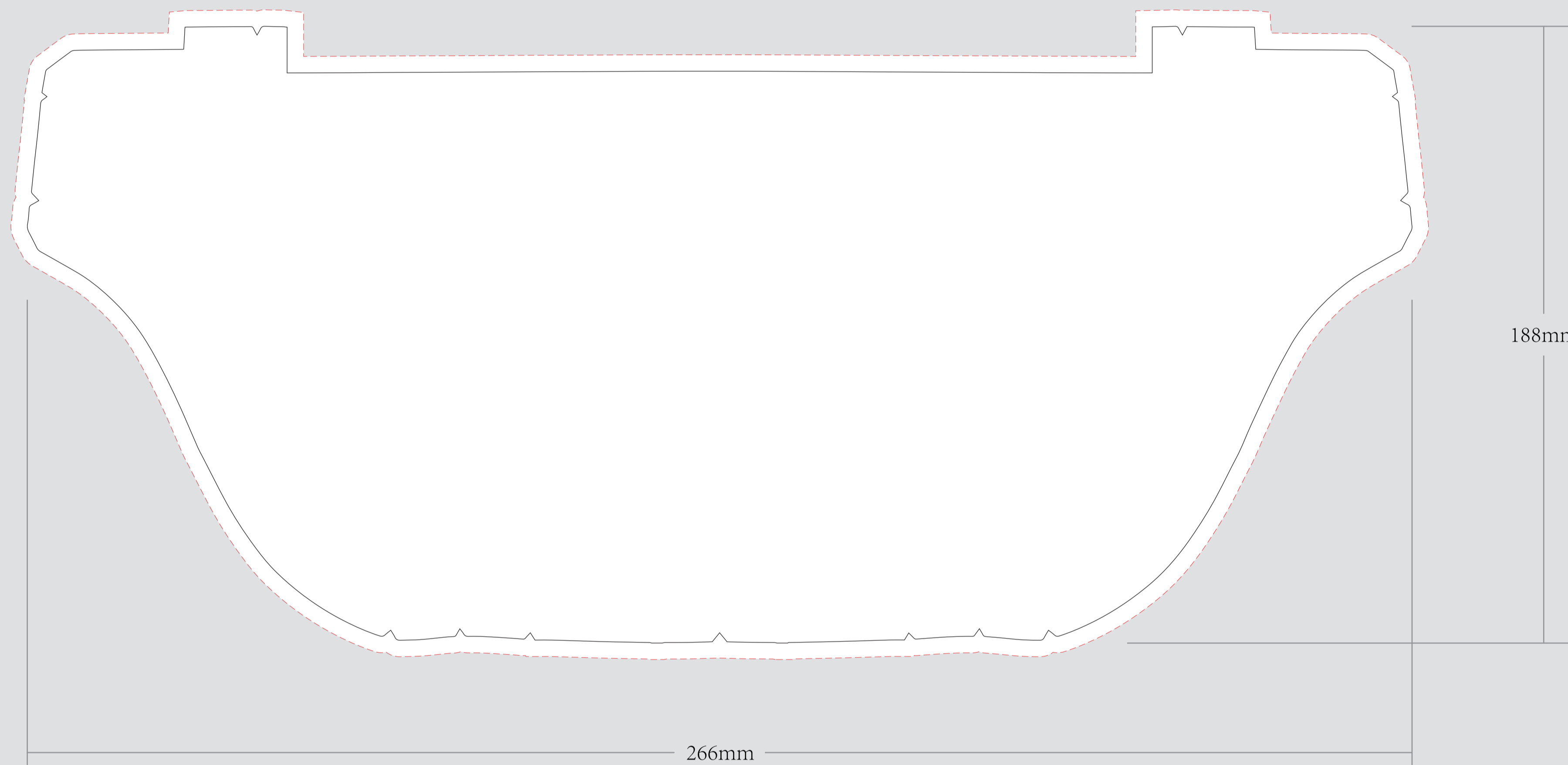
FRONT
