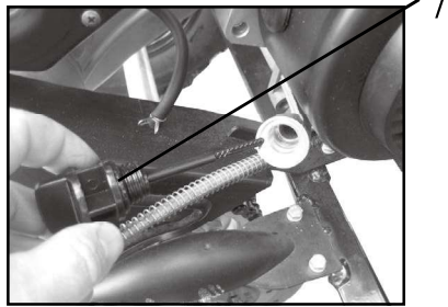
OilFillplug/Dipstick (7)
