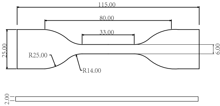
Tensile testing specimen; ASTM D638 (ISO 527, GB/T 1040)
