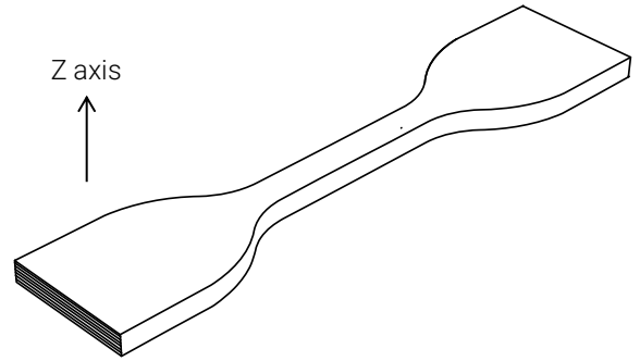
Tensile testing specimen; ASTM D638 (ISO 527, GB/T 1040)
