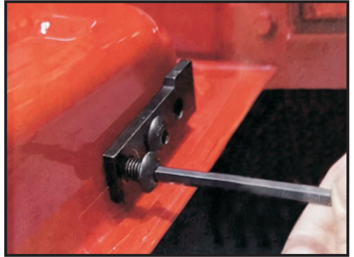
8. Insert only 2 bolts through the bracket. The third bolt shall be installed later in step 12.
