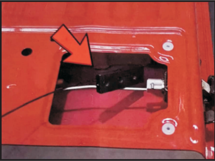
7. Place the backing plate inside your tailgate.
