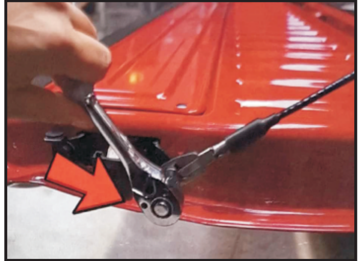
2. Remove strap bolt from the tailgate.
