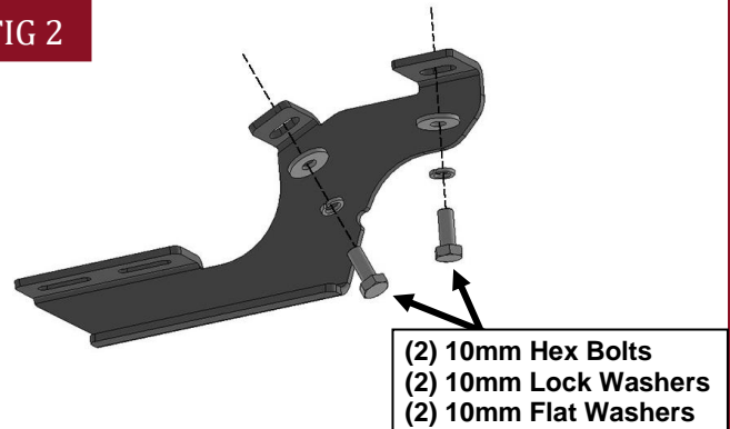
(Fig 2) Attach (1) Front Mounting Bracket to the front location
