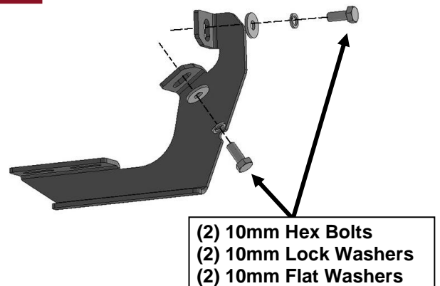
(Fig 3) Attach (1) Center/Rear Mounting Bracket to the center and rear locations
