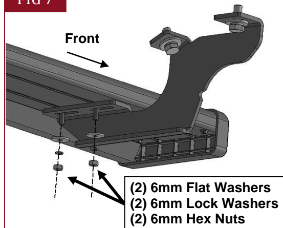
(Fig 7) Attach a Running Board to the Mounting Brackets
