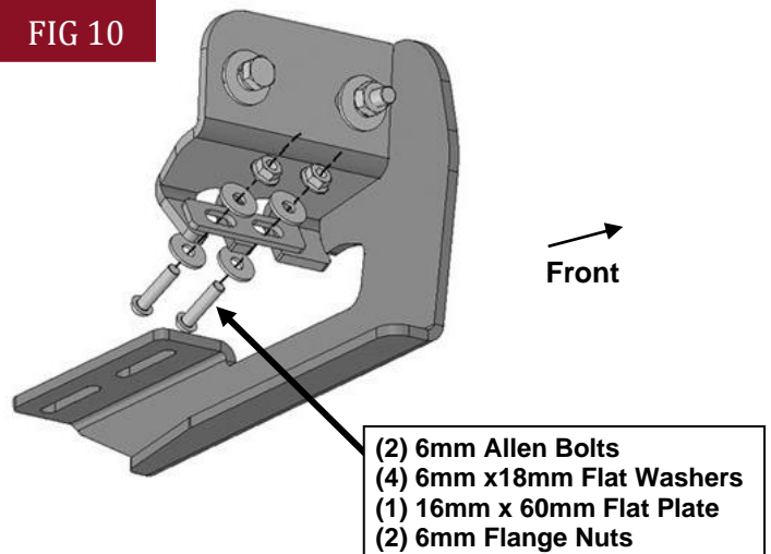
(Fig 10) Attach the Bracket to back of pinch weld, rear shown here, (models with factory holes in pinch weld only)
