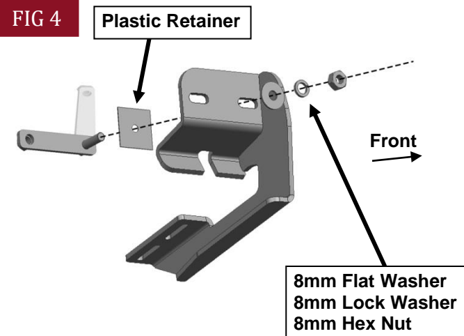
(Fig 4) Attach Driver/Left Front Bracket to 8mm Bolt/Nut Plate.
