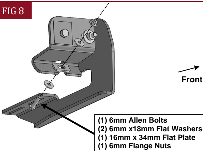
(Fig 8) Attach the Bracket to back of pinch weld, front shown here, (models with factory holes in pinch weld only)
