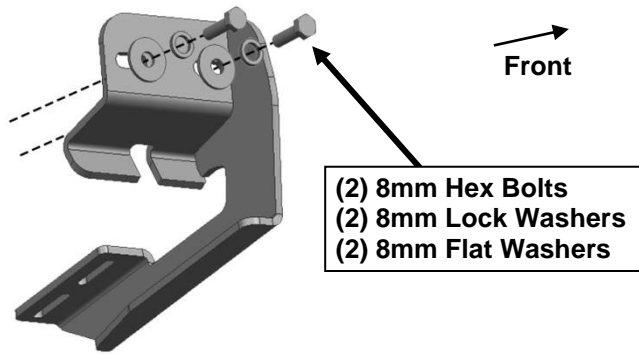
(Fig 7) Driver/left side front models with factory installed threaded inserts. Bolt Plate not required
