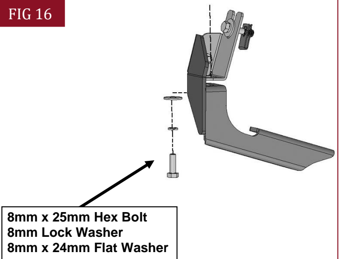
(Fig 16) For models with welded nut in the pinch weld
