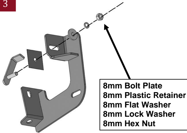
(Fig 3) Attach Driver/Left Bracket to 8mm Bolt Plate
