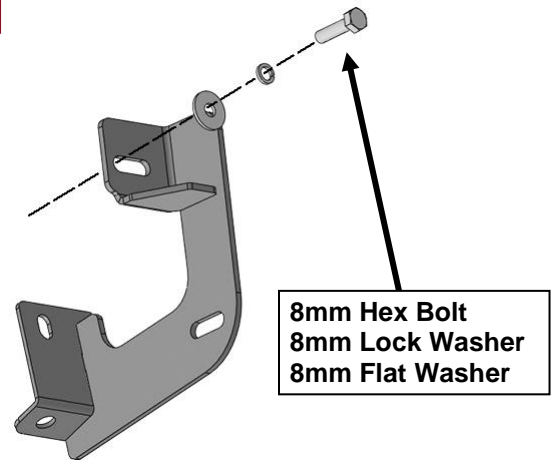
(Fig 5) Attach Driver/Left Mounting Bracket to factory installed threaded inserts
