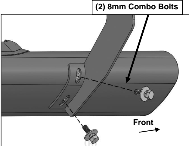
(Fig 12) Sidebar attached to Bracket illustrated
