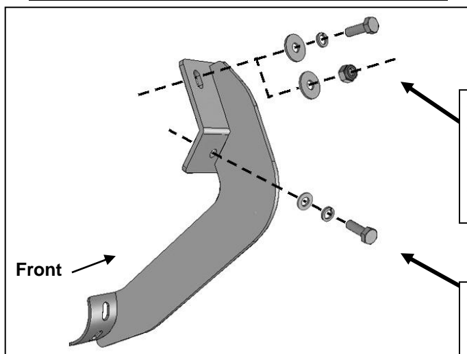
(Fig 2) Driver/left Bracket illustrated for example only
