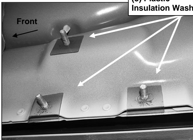
(Fig 3) Thread Plastic Washers onto all mounting studs. Passenger side rear pictured
