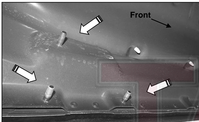
(Fig 1) Locate the (3) factory threaded studs at each location. Driver side rear pictured
