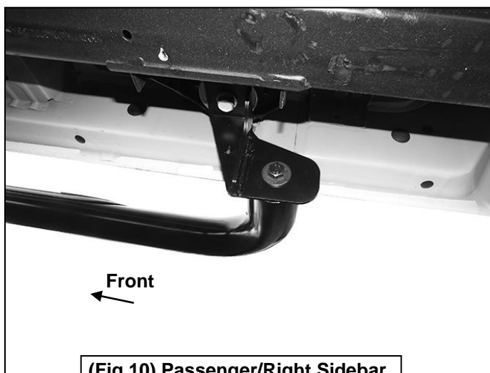
(Fig 10) Passenger/Right Sidebar to the Rear Mounting Bracket
