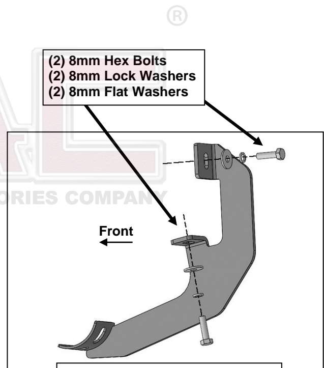
(Fig 3) Attach (1) Mounting Bracket to the mounting location
