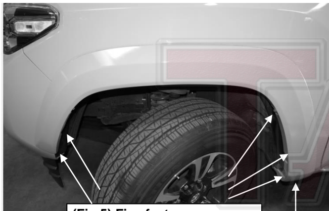
(Fig 5) Five factory screws, driver's side front
