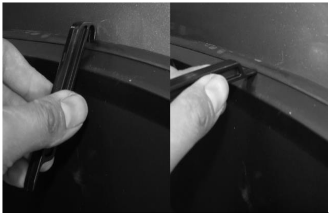
(Fig 20) Use hooked end along vehicle/rubber trim perimeter. Use flat end along rubber trim/flare perimeter
