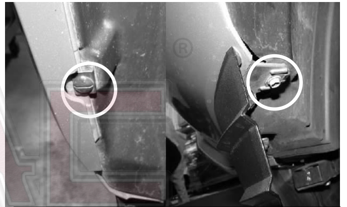
(Fig 6) Left: Remove fastener (can pry it out with screwdriver), Right: Remove fastener on the bottom.
