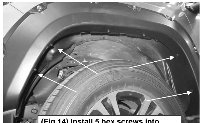
(Fig 14) Install 5 hex screws into remaining mounting holes
