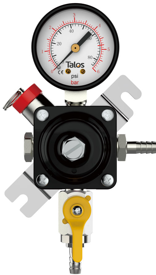
Single Gauge With Barbs And Plug 1077319
