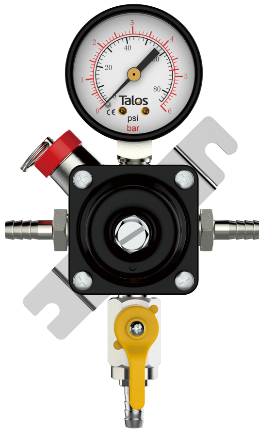
Single Gauge With Two Barbs 1077308
