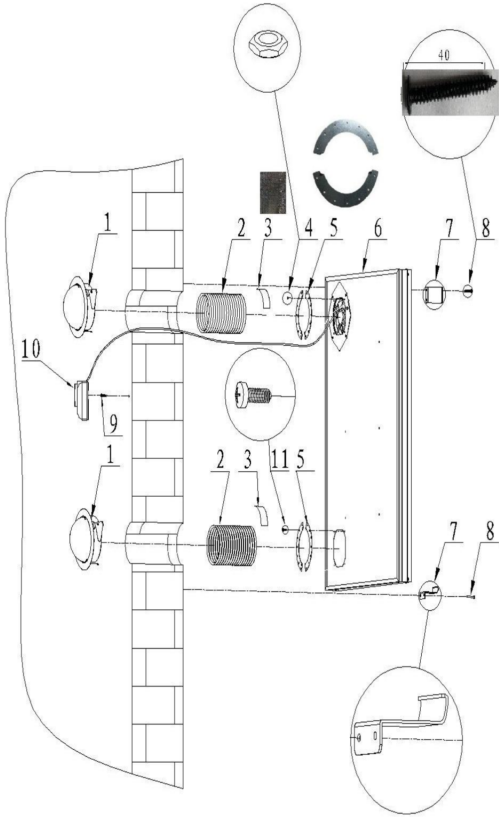
OS22, OS32, OS42 with mechanical thermostat
